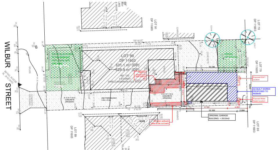
SITE PLAN
