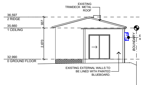
SOUTH ELEVATION
