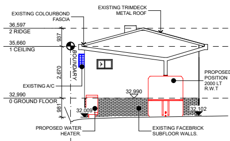
NORTH ELEVATION
